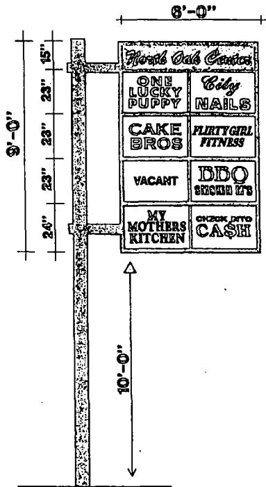
9'x6' FLAG MOUNT POLE SIGN
