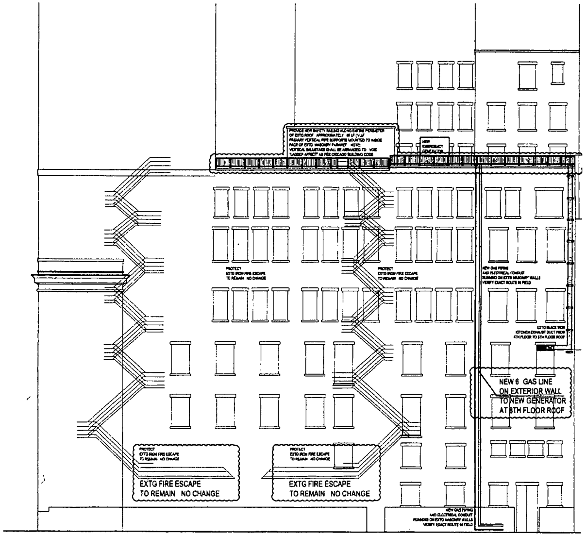
2 REAR ALLEY - WEST SIDE - EXTERIOR ELEVATION DETAIL SCALE 3/16" = 1'-0"
