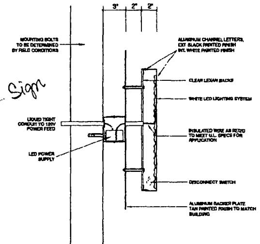
SILHOUETTE INTERNALLY ILLUM. CHANNEL LTR. DETAIL
