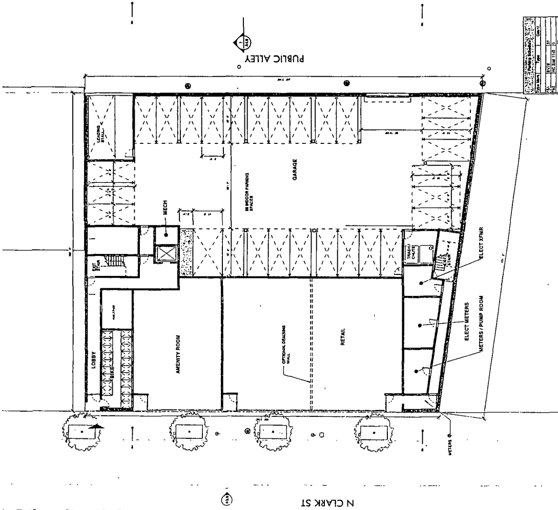
2. Ground Floor Plan 1/8" = 1'-0"
