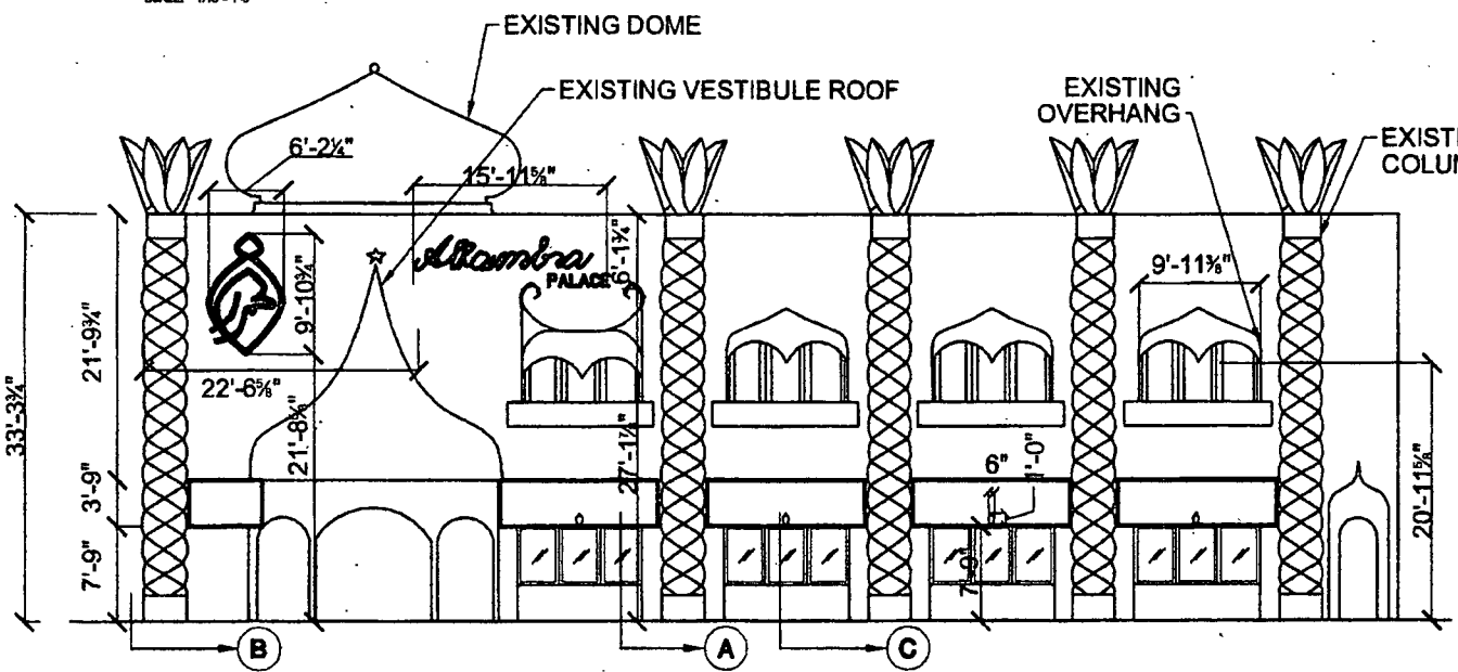
2 SOUTH ELEVATION SCALE: 1/16" = 1'-0"
