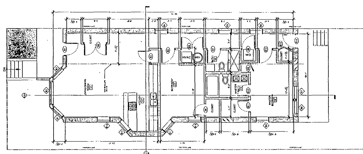
1 BASEMENT CONSTRUCTION PLAN 1/4" = 1'-0"
