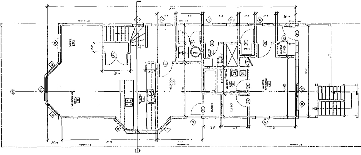
1 SECOND FLOOR CONSTRUCTION PLAN 1/4" = 1'-0"
