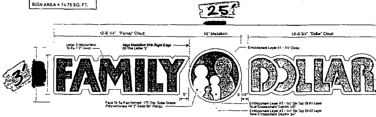
Front View - 34.5" Linear Cloud / 46" Medallion Scale: 3/8" = 1'-0"
