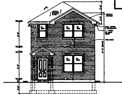
FRONT ELEVATION 1/8" = 1'-0"
