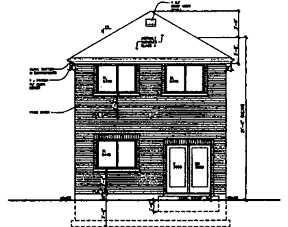
REAR ELEVATION 1/8" = 1'-0"
