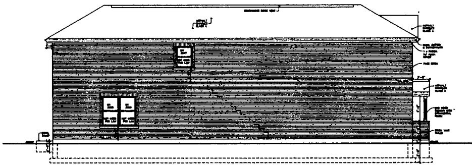
LEFT SIDE ELEVATION 1/8" = 1'-0"
