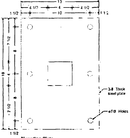
Mounting Plate 3/8" Re Use existing bottom plate attachment holes New plate and mounting at top of blade sign
