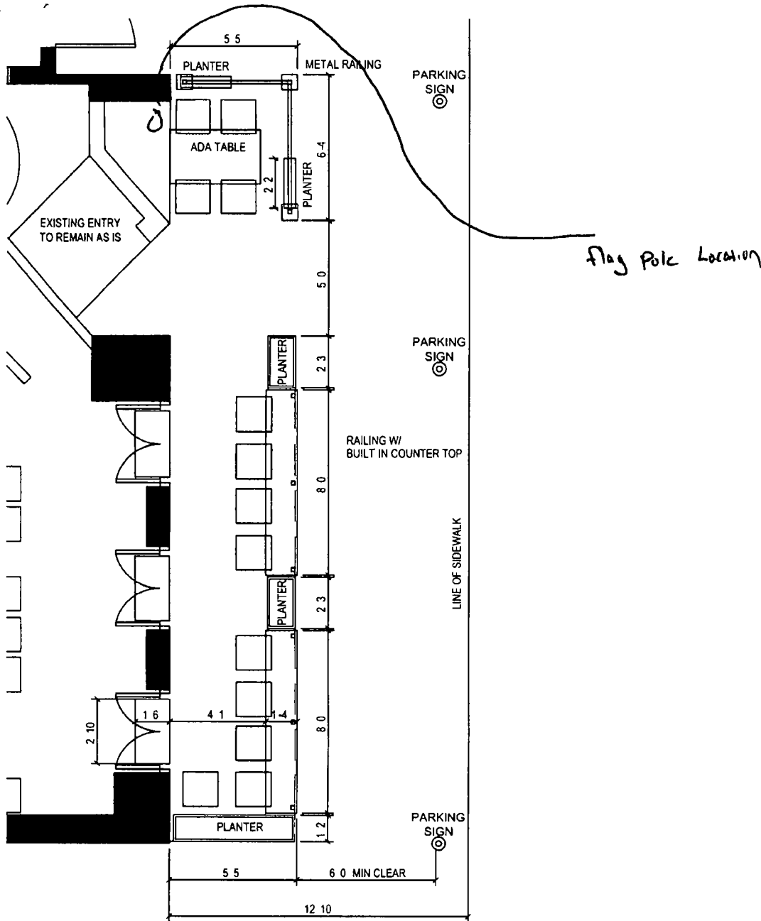
SIDEWALK CAFE PLAN SCALE 3/16" = 1'-0"
