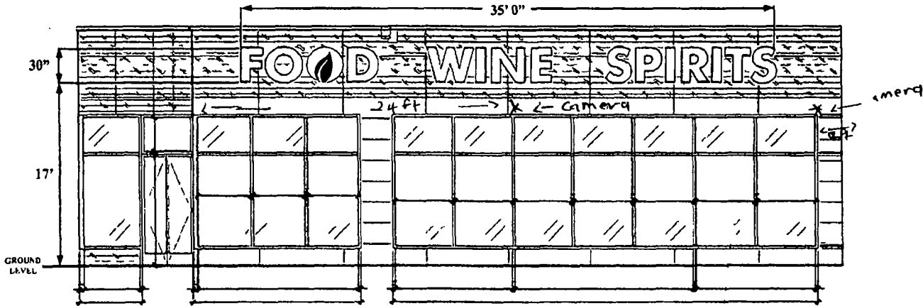
WEST IRVING PARK ROAD ELEVATION
