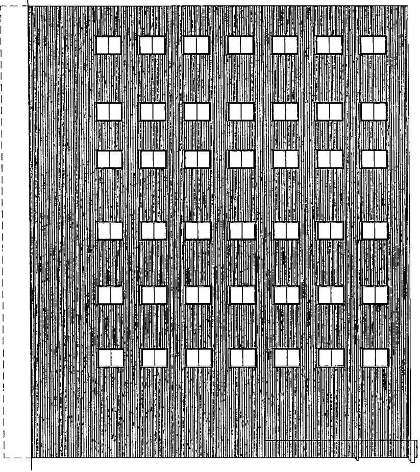
EXISTING SOUTH ELEVATION 1/8" = 1'-0" 5' 0" 5' 10' 20' 40'
