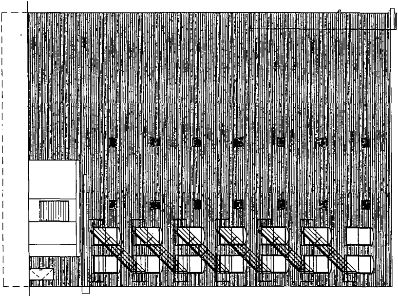
EXISTING WEST ELEVATION 1/16" = 1'-0" 5' 0" 5' 10' 20' 40'
