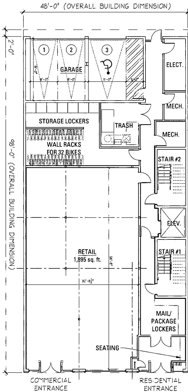
FIRST FLOOR PLAN - 3,993 SF
