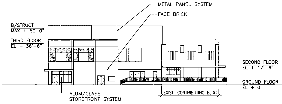
1 EAST ELEVATION SCALE 1" = 40'-0"
