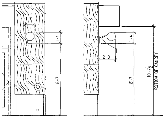
3 SCONCE FRONT & SIDE ELEVATION
