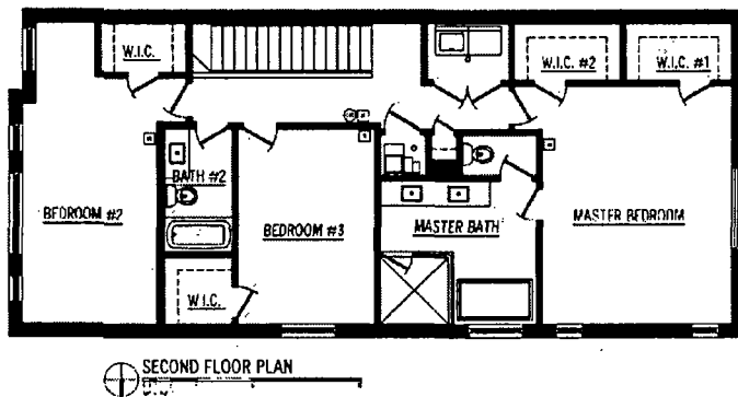
Proposed Elevations and Floor Plan 3300 S. Giles Avenue (Source: Three Sixty Design Studio, LLC)
