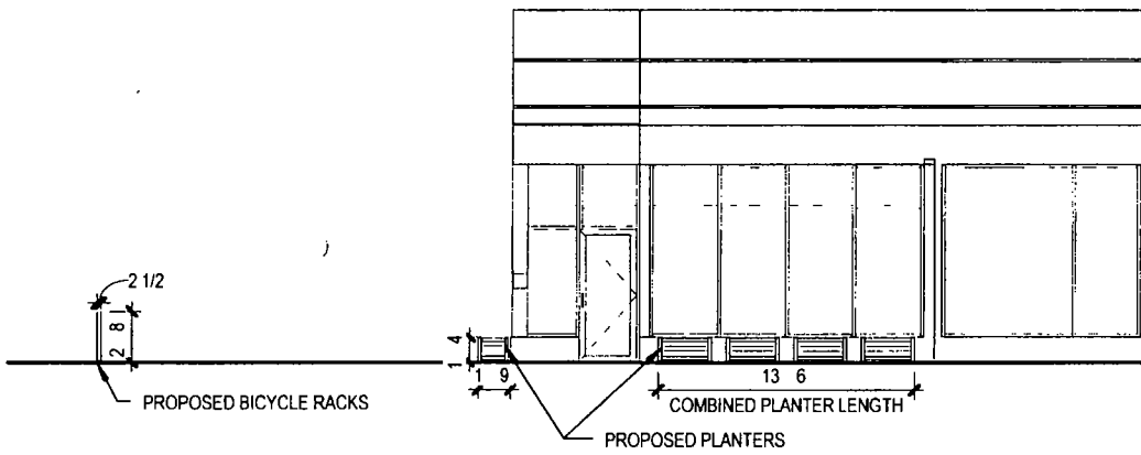
① PROPOSED NORTH ELEVATION 1/8" = 1'-0"
