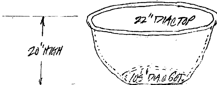
PROPOSED PLANTER DETAIL (NTS)
