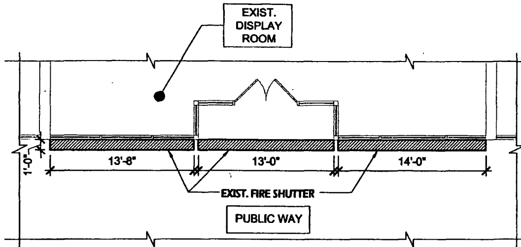
EXIST. FIRE SHUTTER LAYOUT SCALE: 1/8" = 1'-0"
