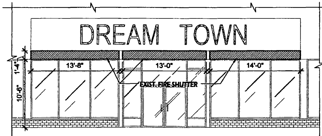
EXIST. FRONT ELEVATION SCALE: 1/8" = 1'-0"
