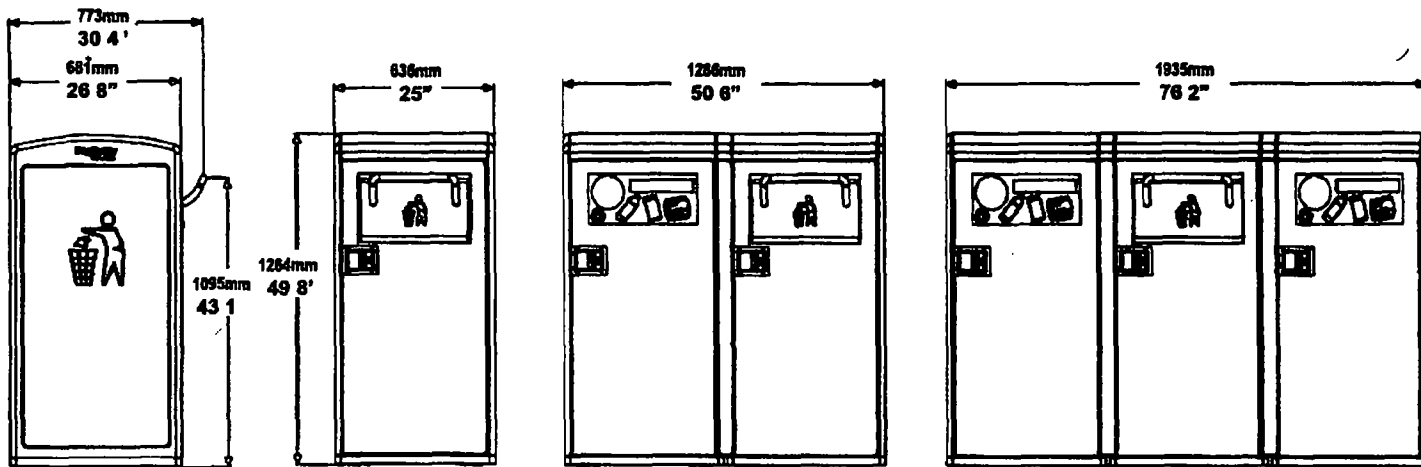
Bigbelly single station Approximately 270 lbs (123kg)
