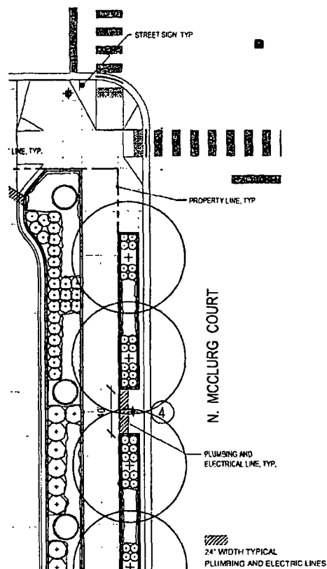
MCCLURG STREET-NORTH: PLANTERS ELECTRIC AND PLUMBING LINES
