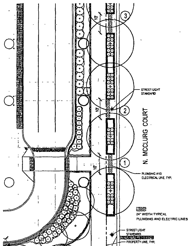
MCCLURG STREET-SOUTH: PLANTERS ELECTRIC AND PLUMBING LINES
