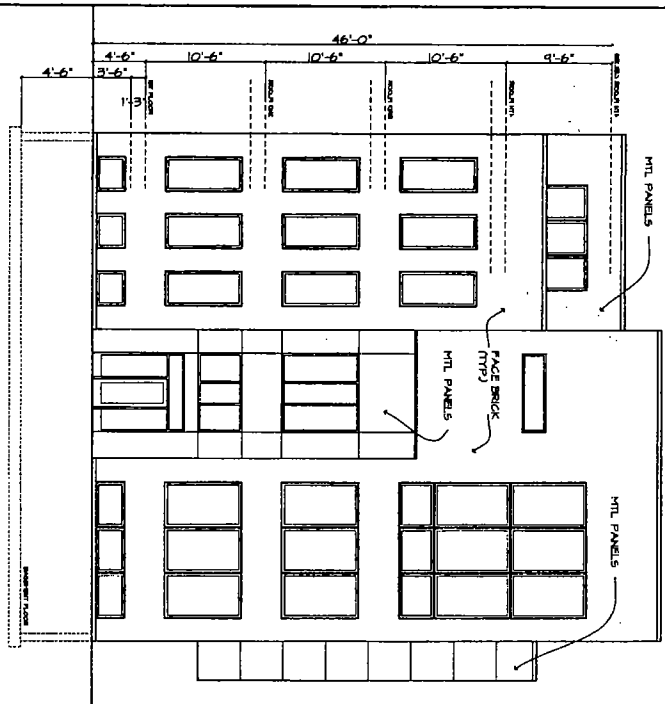
FRONT ELEVATION
