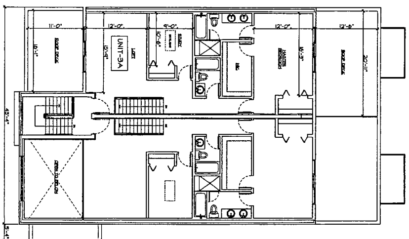
4TH FL. PLAN
