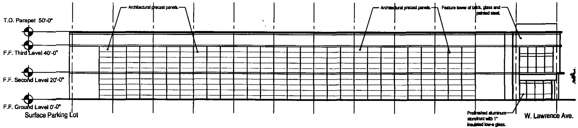
West Elevation - Chicago and Northwestern Railway
