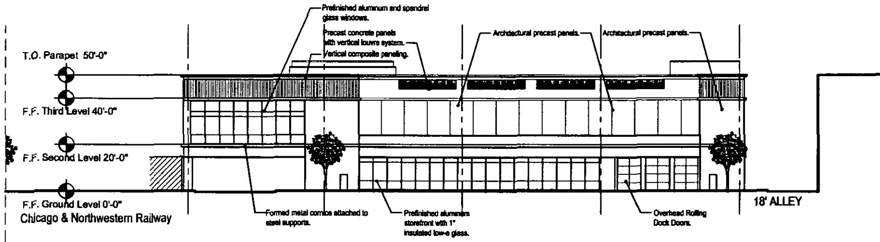
North Elevation - Lawrence Avenue
