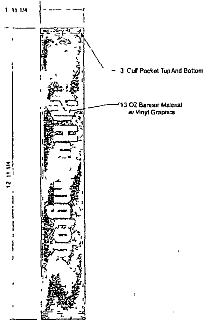
FRONT ELEVATION FLAG BANNER SCALE 1/2" = 1'-0" (1 Required)
