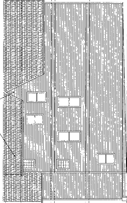
2 EAST ELEVATION SCALE: 3/4" = 1'-0"
