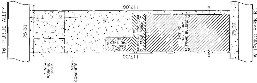
2 PROPOSED SITE PLAN
