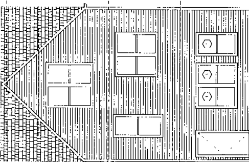
1 SOUTH ELEVATION SCALE: 3/4" = 1'-0"
