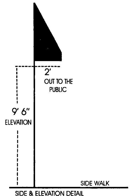
SIDE & ELEVATION DETAIL
