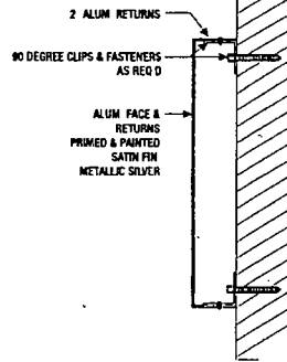
N/O FABRICATED ALUM LETTERS SECTION DETAIL
