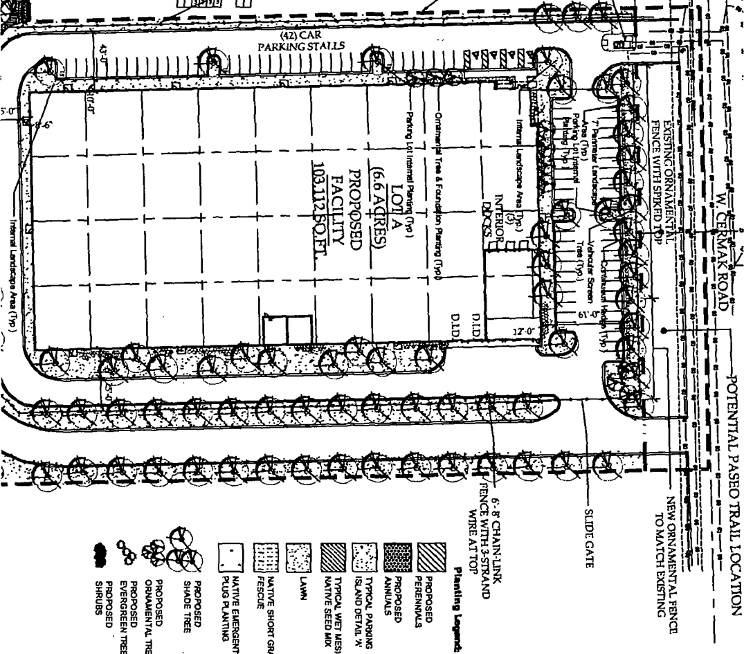
Enlarged Planting Detail (LP-1)
