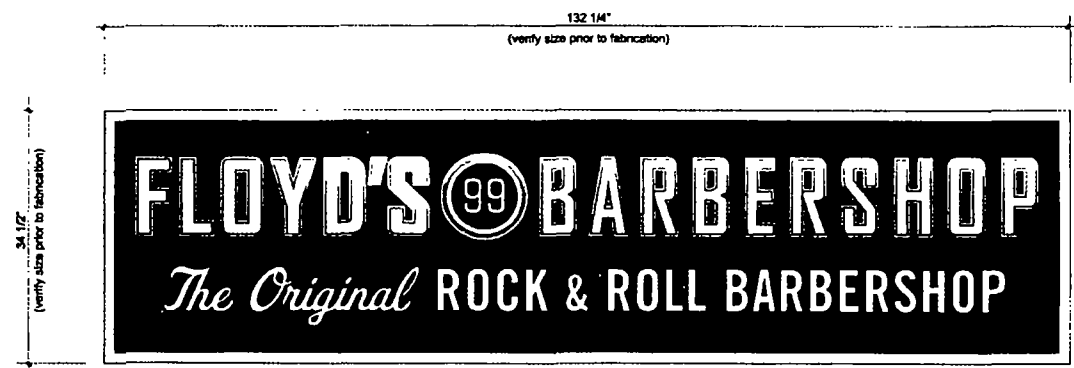
Single Faced Cabinet Sign Elevation-1"x1'-0"
