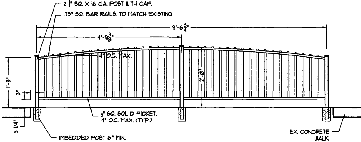
1 WELDED ORNAMENTAL METAL RAILING IN TREE PIT NOT TO SCALE
