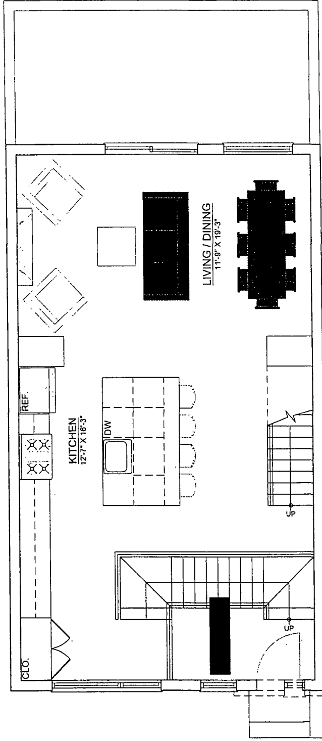
1 1ST FL. ENTRY / 2ND FL. PLAN - TOWNHOME #1 1/4" = 1'-0"
