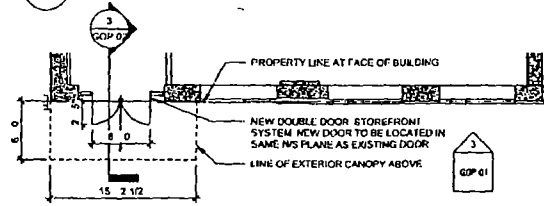
2 LEVEL 1 - ENLARGED PLAN SOUTH ENTRANCE
