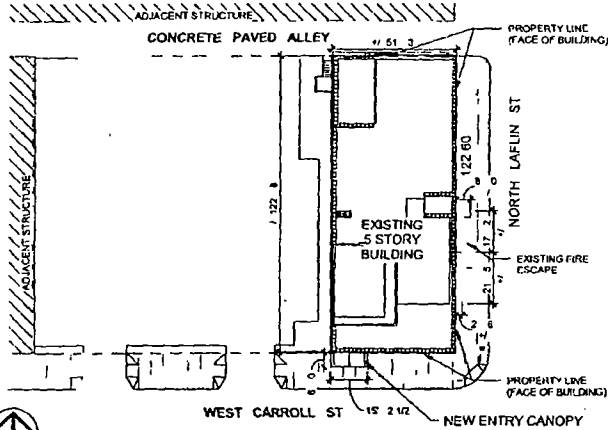
1 SITE PLAN
