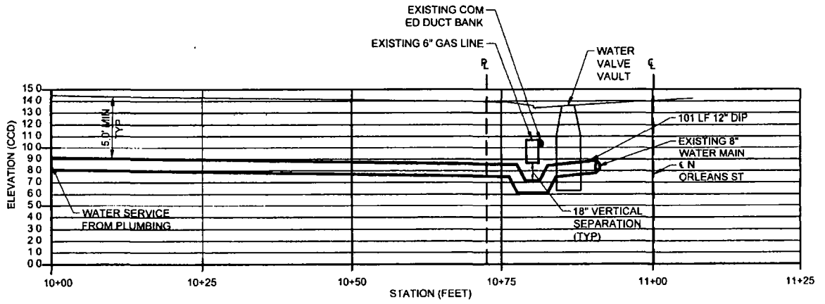
6 WATER SERVICE PROFILE SCALE V 1"=5 H 1"=10
