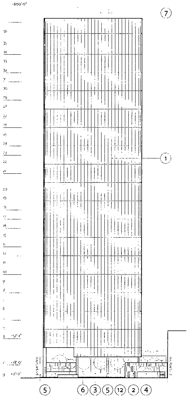
Sub Area A South Elevation Scale: 1" = 80'-0"
