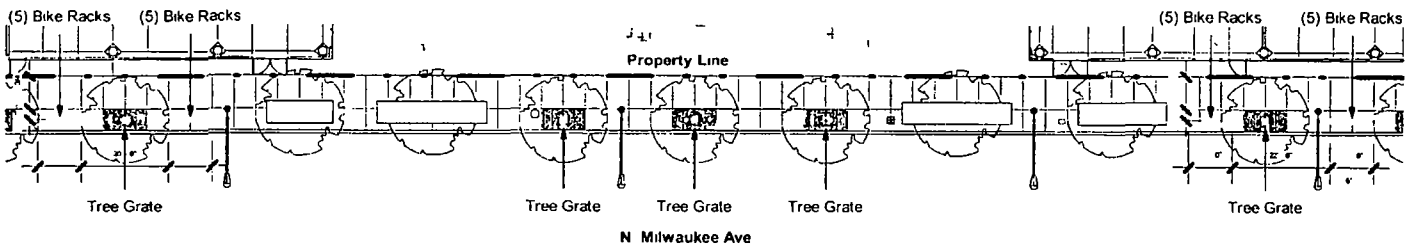
② Sidewalk Plan - Bike Rack 1" = 40'-0"
