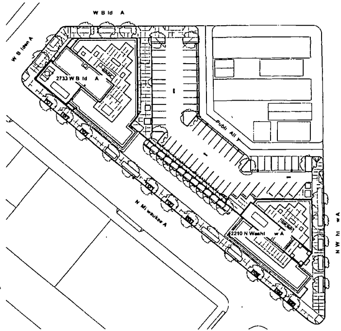
③ Site Plan - Public Way Permit - Bike Rack 1" = 100'-0"
