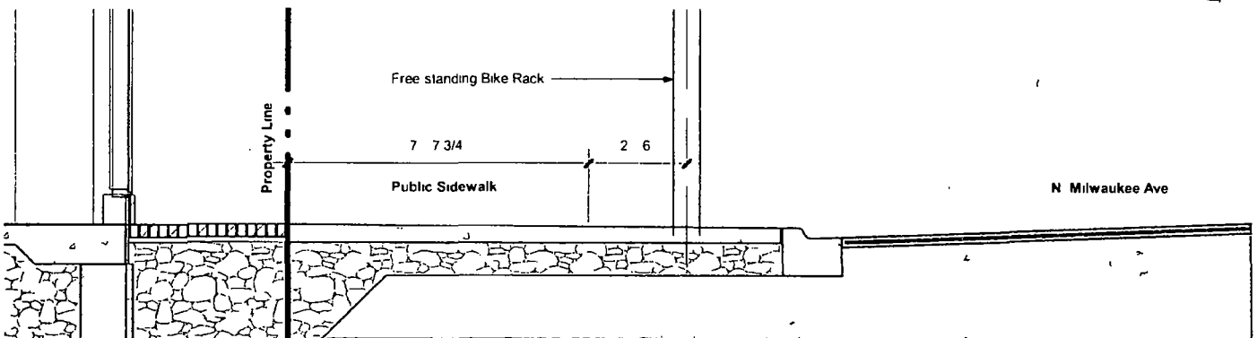
① Public Way Section - Bike Rack 1/4" = 1'-0"
