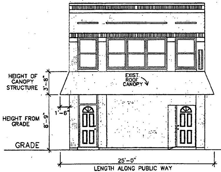
EXISTING CANOPY ONE FRONT ELEVATION
