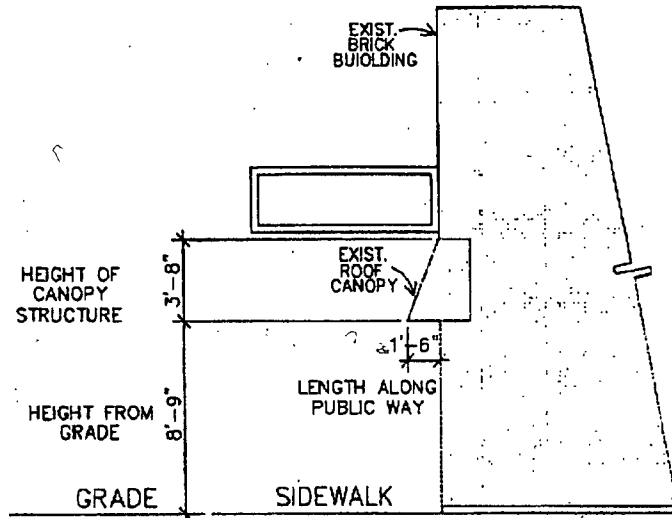
EXISTING CANOPY ONE SIDE VIEW
