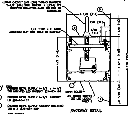
RACEWAY DETAIL
