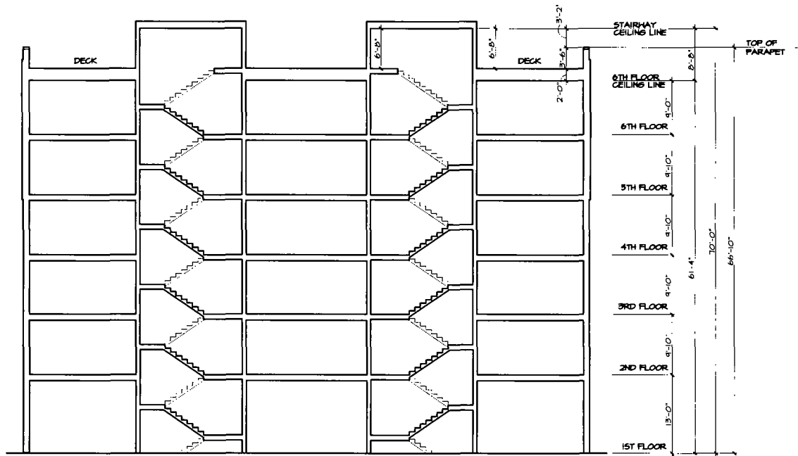
BUILDING SECTION
