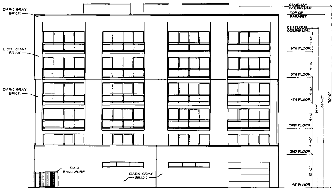
NORTH ELEVATION
