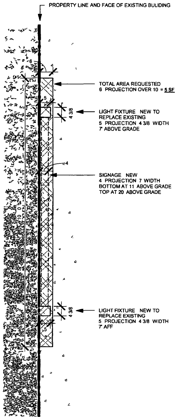
② Enlarged Plan showing projections into PROW 1/2" = 1'-0"
