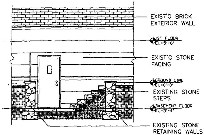
AREAWAY LONGITUDINAL SECTION B-B
