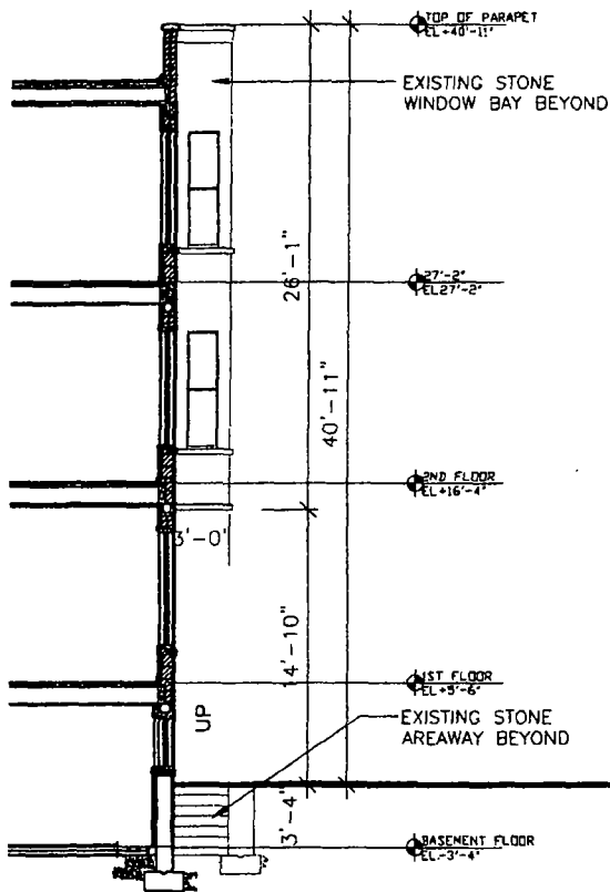
EXT. WALL SECT. A-A 1/8"=1'-0"
