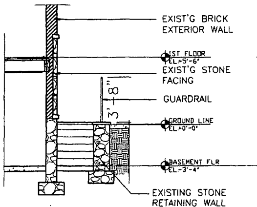
AREAWAY CROSSECTION C-C
