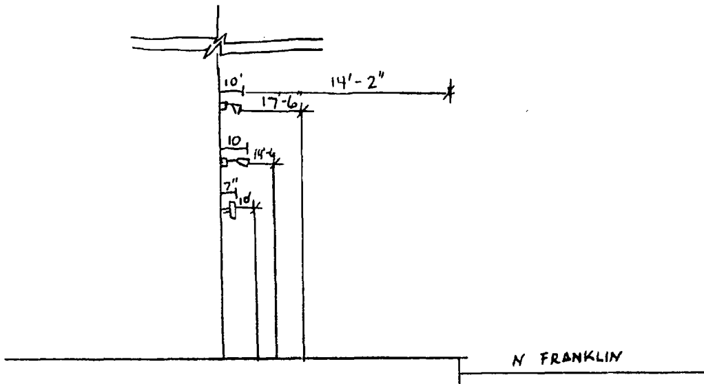
WEST ELEVATION - LIGHT FIXTURE NTS
