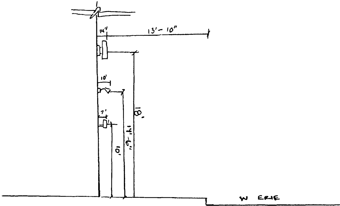
SOUTH ELEVATION - LIGHT FIXTURE NTS
