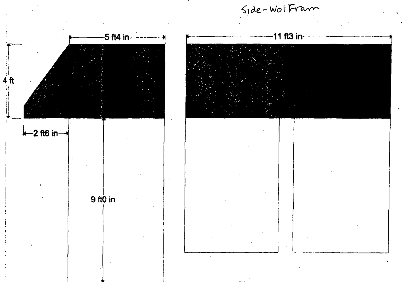
South Elevation
