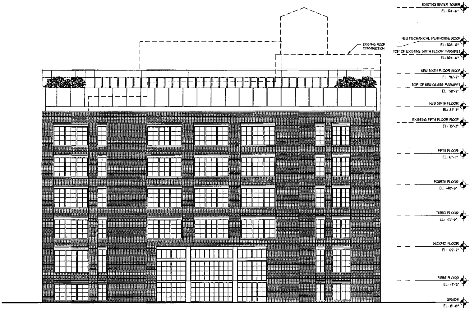
1 EAST ELEVATION SCALE: 1/16" = 1'-0"
