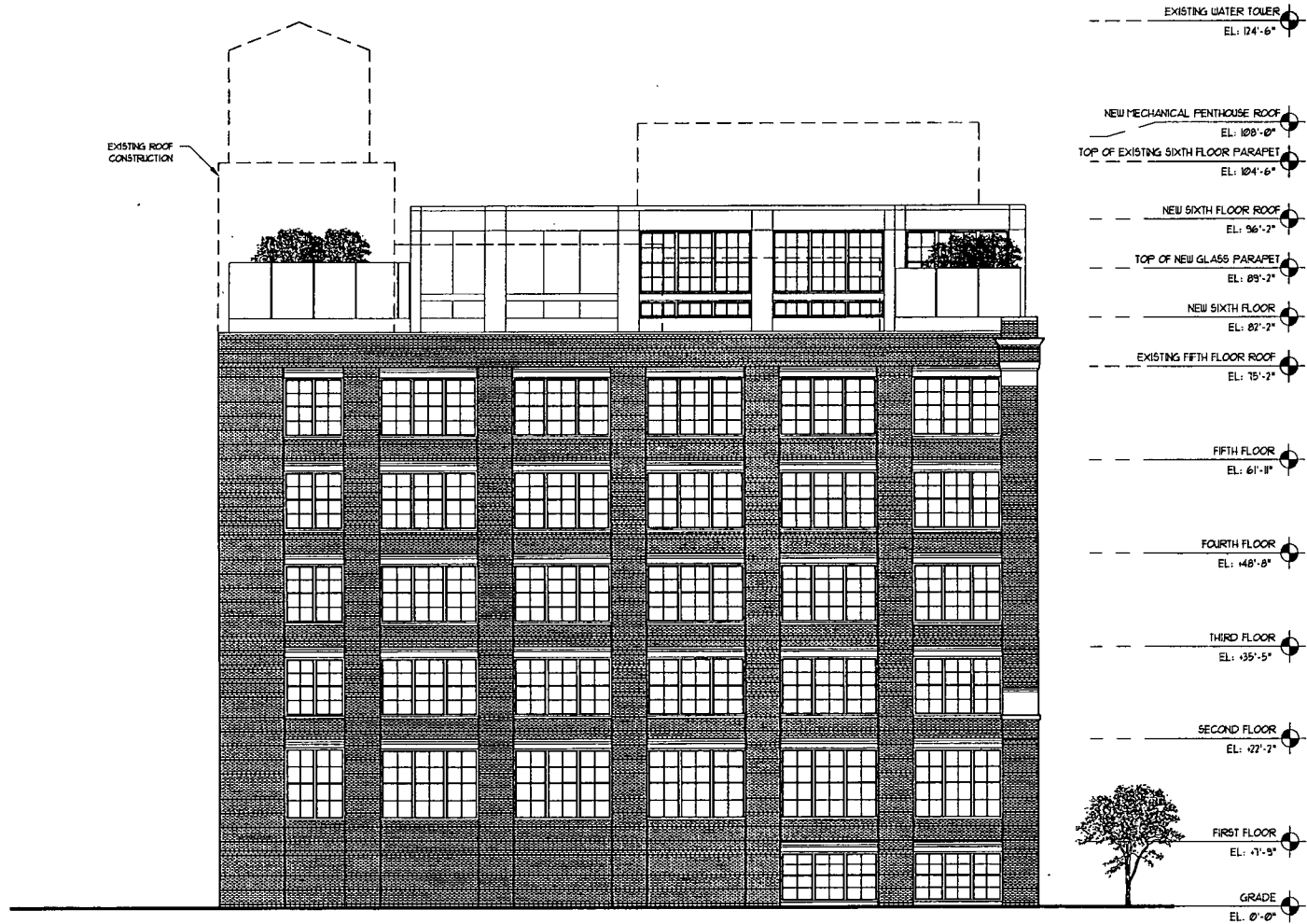
1 NORTH ELEVATION SCALE: 1/16" = 1'-0"
