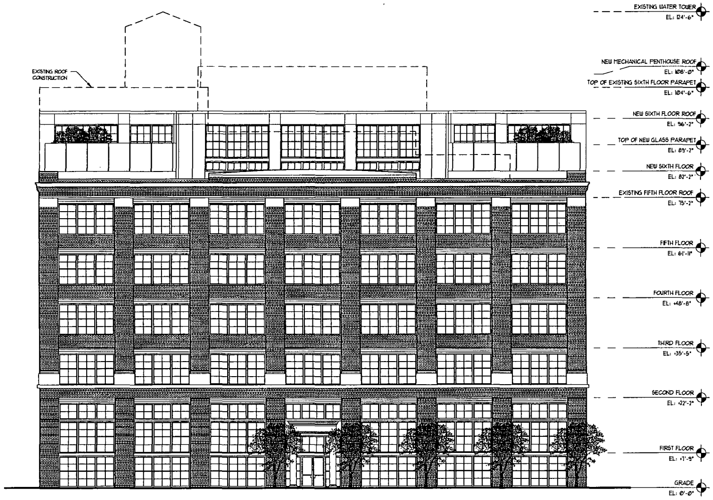
1 WEST ELEVATION SCALE: 1/16" = 1'-0"
