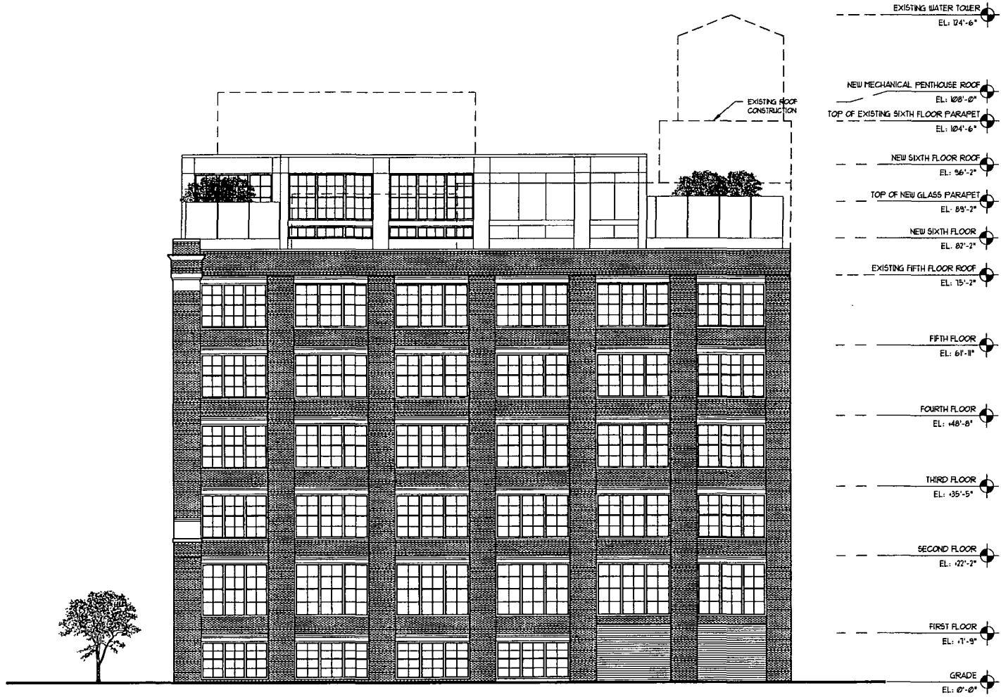
1 SOUTH ELEVATION SCALE: 1/16" = 1'-0"
