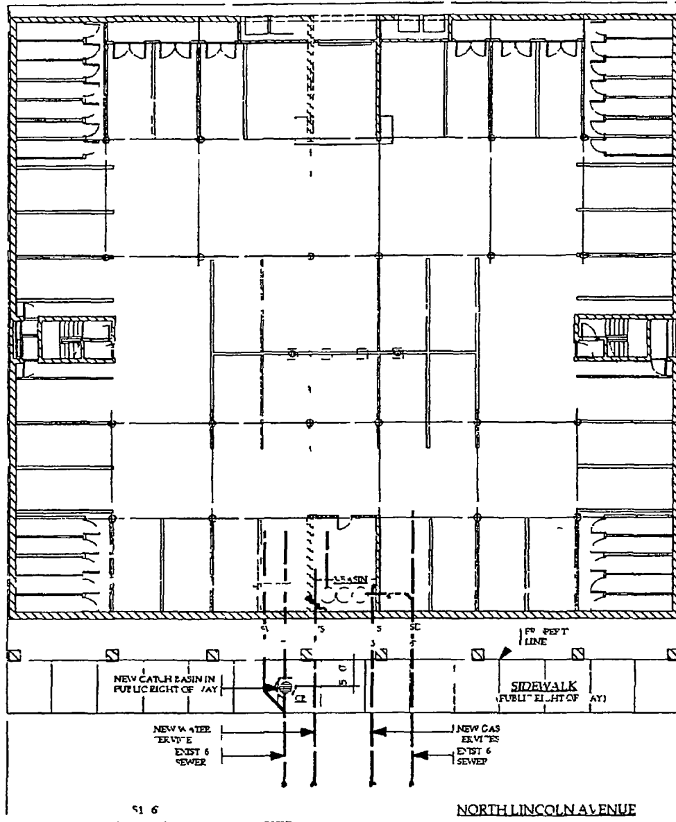
(A) LOWER LEVEL PLUMBING, MECHANICAL & ELECTRICAL PLAN
