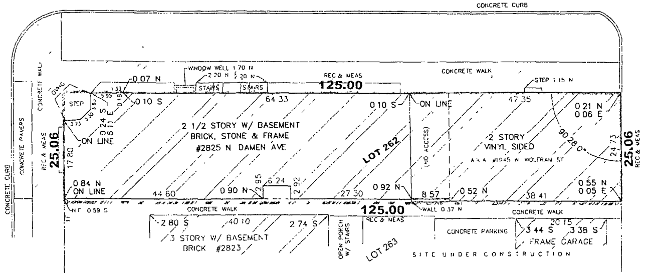
SITE PLAN 1" - 15'
