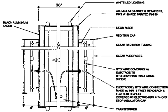
SECTION DETAIL THRU LETTERS & LOGO
