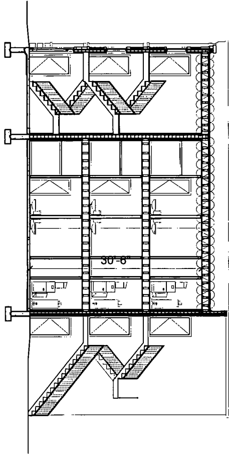
1 BUILDING SECTION Scale: A1/S
