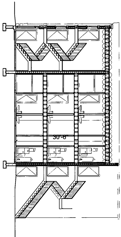
1 BUILDING SECTION Scale: 1/8" = 1'-0"
