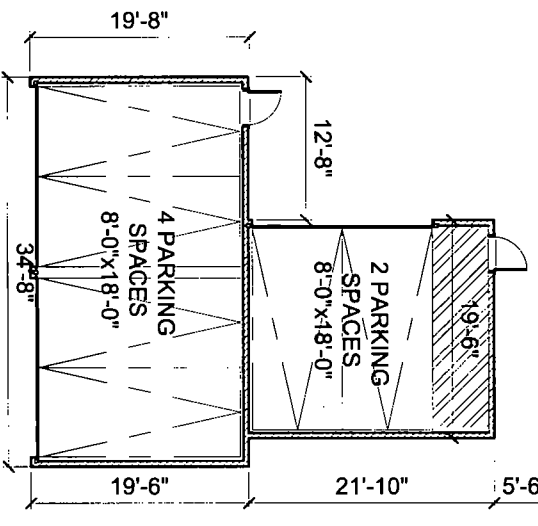
FIRST FLOOR PLAN Scale N.T.S.
