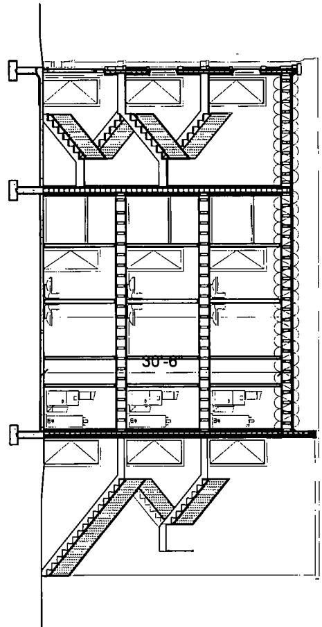
1 BUILDING SECTION P5 Scale: 1/8" = 1'-0"
