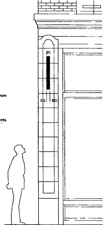
Front Elevation 1/2"=1'-0"
