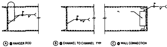
6 TYP. CHANNEL TO CHANNEL CONNECTION SCALE 1/2" = 1'-0"
