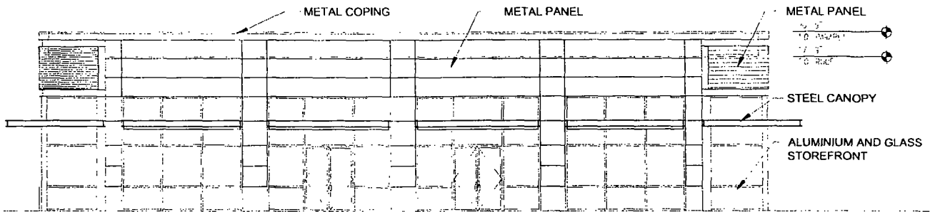
RETAIL A8 - WEST ELEVATION SCALE 1/8" = 1'-0"
