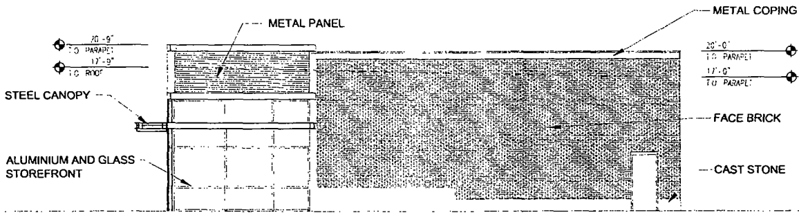
RETAIL A8 - SOUTH ELEVATION SCALE 1/8" = 1'-0"
