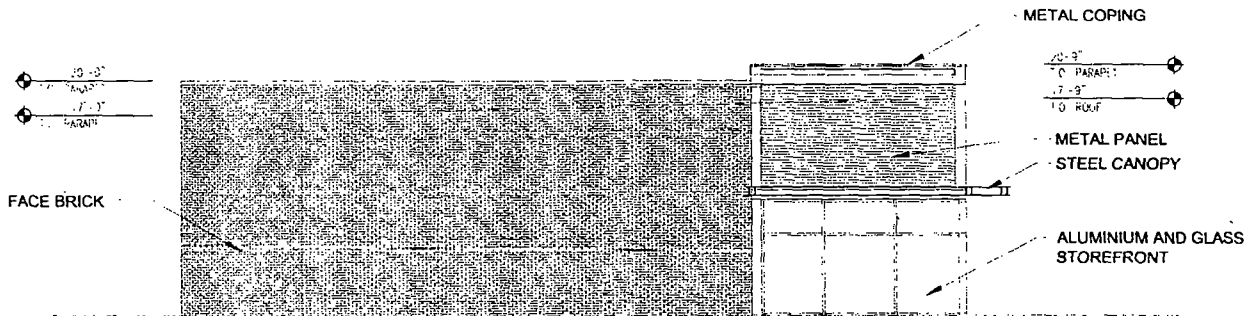
RETAIL A7 - NORTH ELEVATION SCALE 1/8" = 1'-0"
